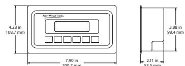
Panel Mount
