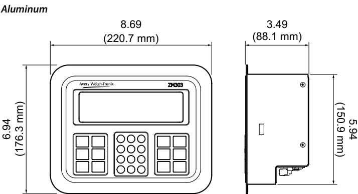
Panel Mount
